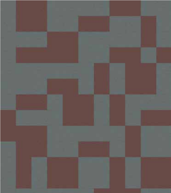
Installation example with 48x48 cm tiles and 24x96 cm planks
